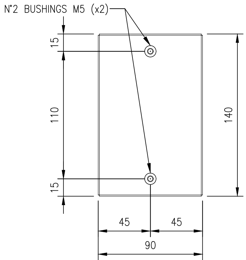
REAR VIEW
