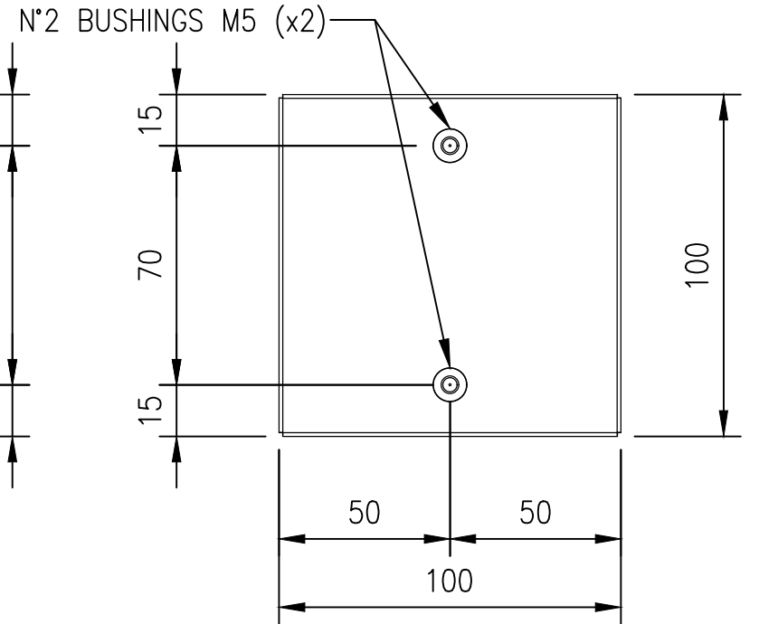
REAR VIEW
