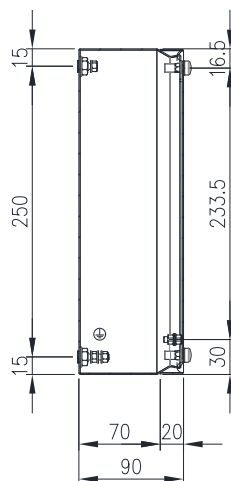
SECTION B-B
