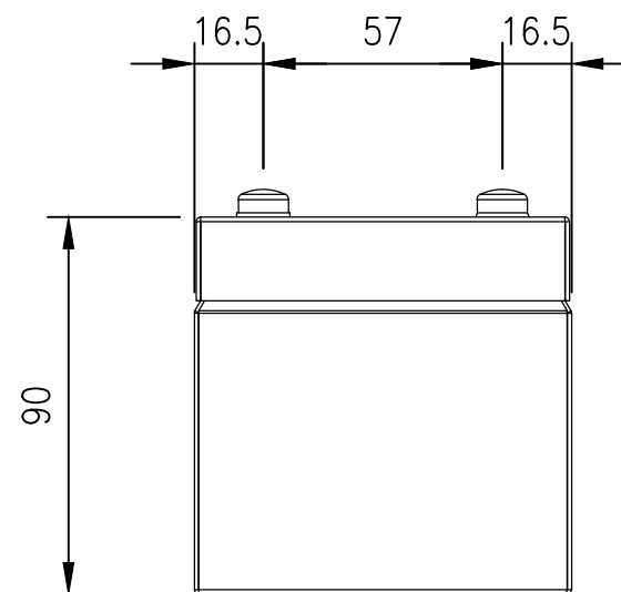
BOTTOM VIEW
