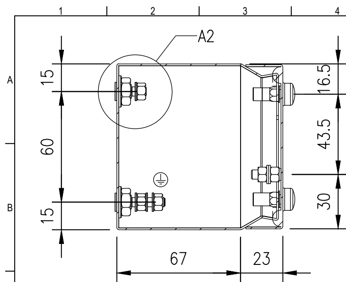
SECTION B-B
