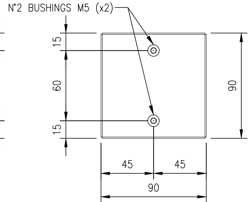
REAR VIEW
